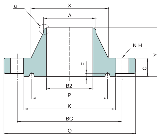
WELDING NECK RTJ
