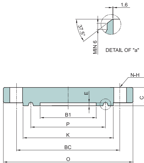
BLIND RTJ
