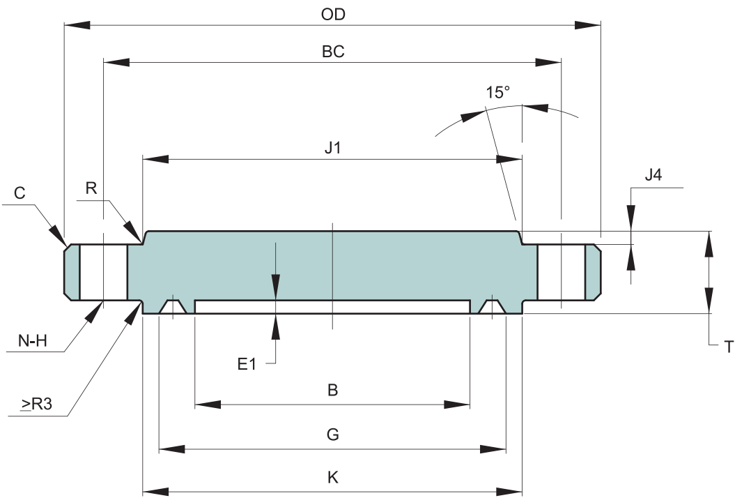
(BLIND RTJ)
