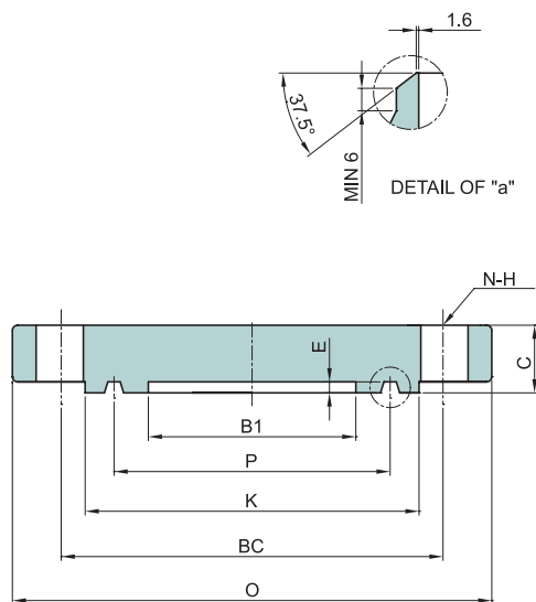
BLIND RTJ
